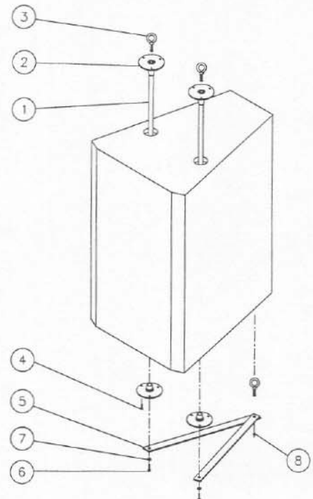
Figure 3—Exploded view of T221 and HST1 parts
